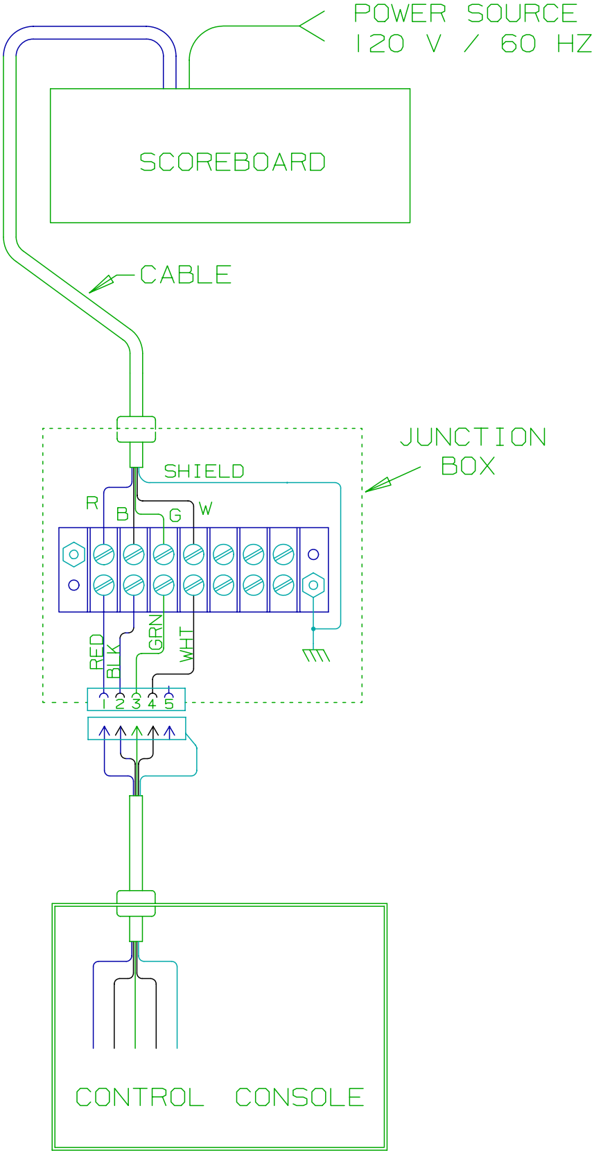
SYSTEM LAYOUT
